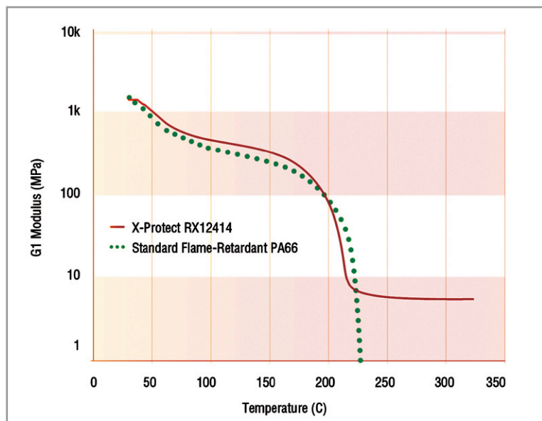
Temperature performance of Ascend’s Starflam X-Protect FR PA66.
