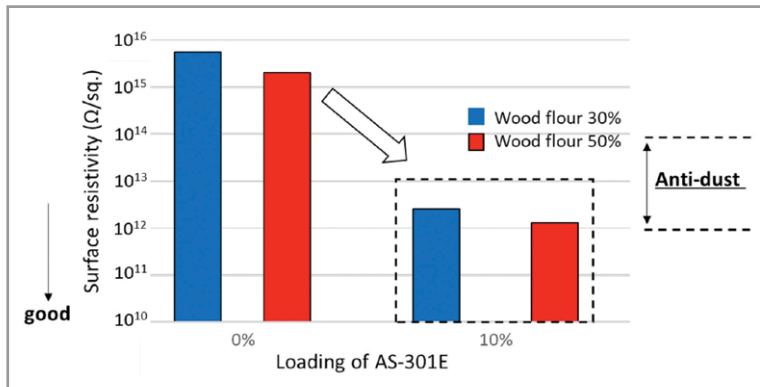
Figure 1: Antistatic performance of PP/wood flour WPCs containing Adeka’s Addstab AS-301E permanent antistat additive
